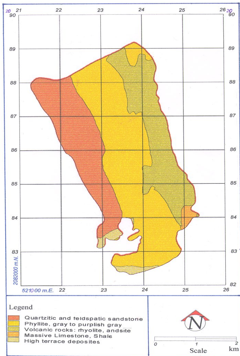
Figure 4 Geologic map of the Huai Hong Khrai Watershed. Sources : Geological Survey Division (1971)
